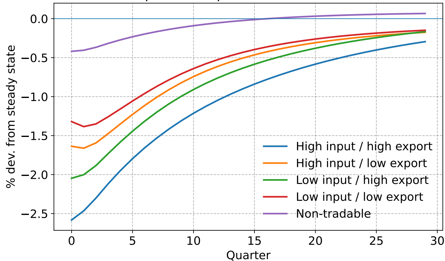
Sector-specific output under the full trade war
